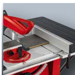
Parallel guide with eccentric clamp and additional cross stop
