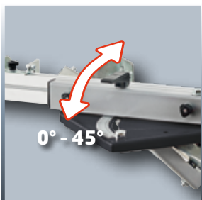
Cross stop with angle setting from 0° to 45°
